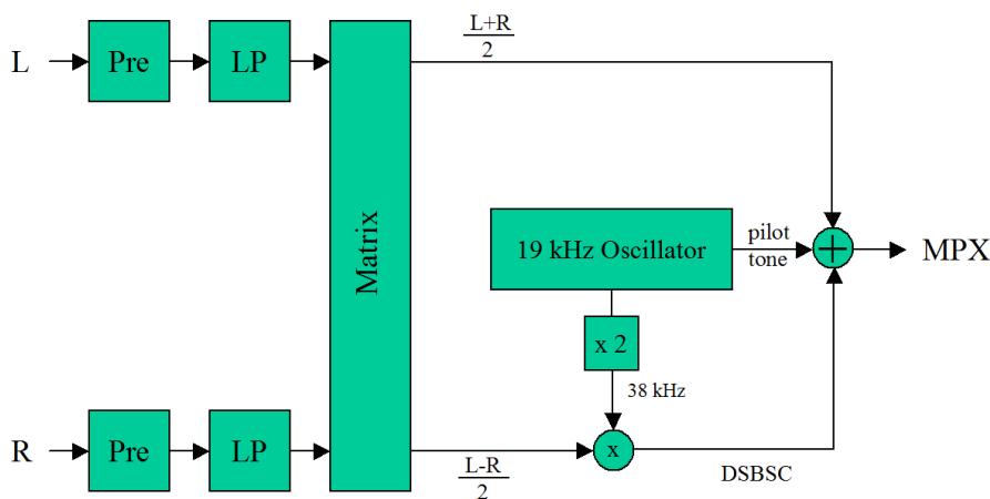
Figure 7 stereo encoder
